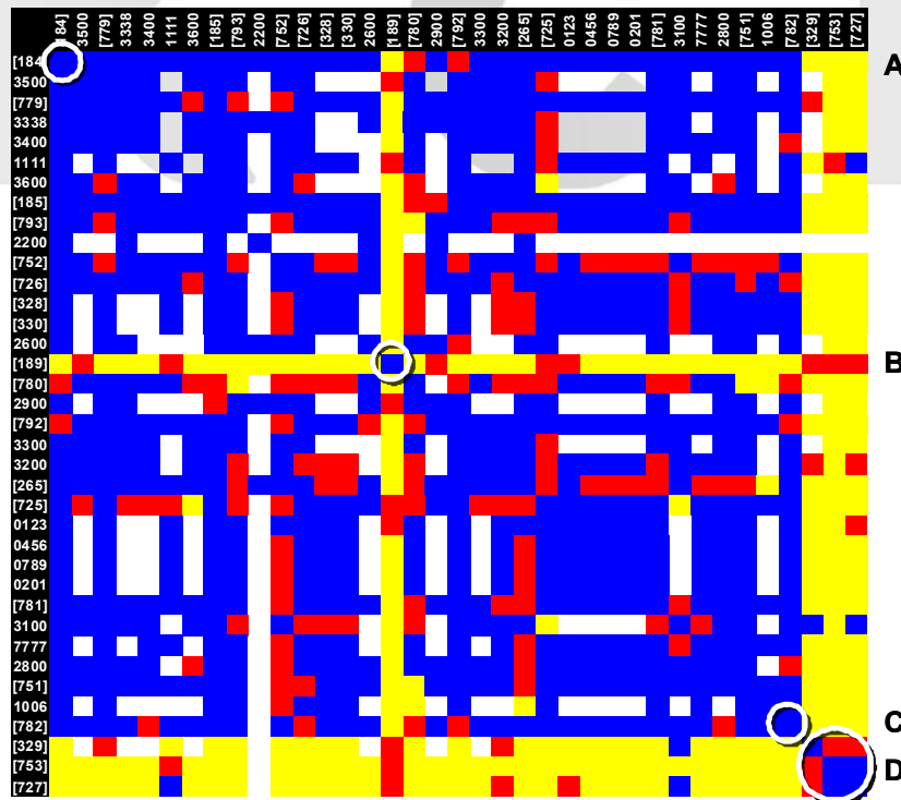
Fig. 2. Correlation matrix of wind speed (■: >0.6, ■: 0.3~0.6, ■: <0.3, □: ND).
