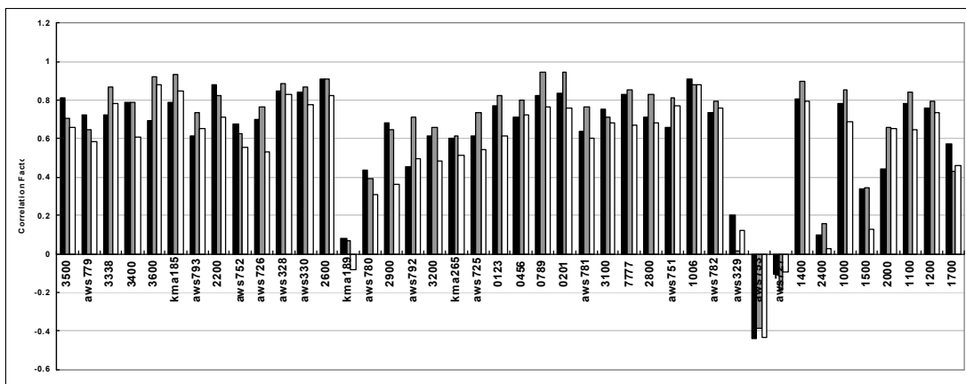
Fig. 3. Comparison of correlation factors of monthly wind speed (upper) and its R-squared (lower) between Jeju weather station(■), Gosan radiosonde data(■: 125 m, □: 3 km a.g.l.) and other in-situ measurements.
