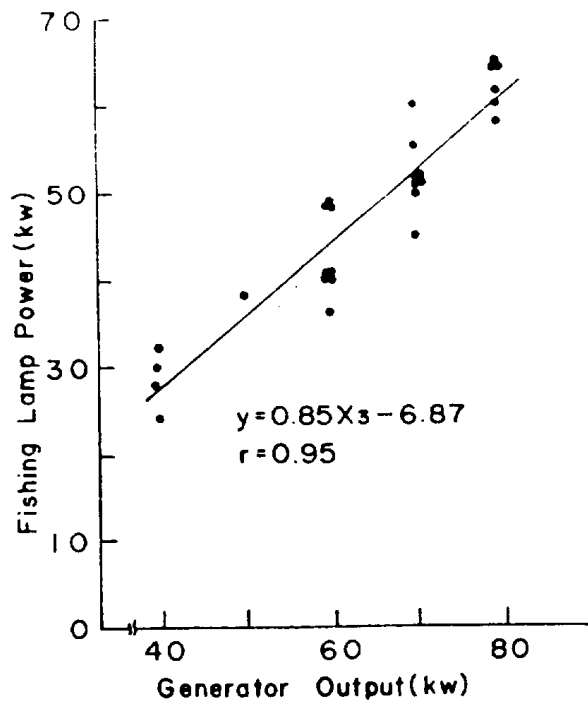
Fig. 12. Relationship between fish lamp power and out put of generator for fishing boat of the ribbon fish line fishing.
