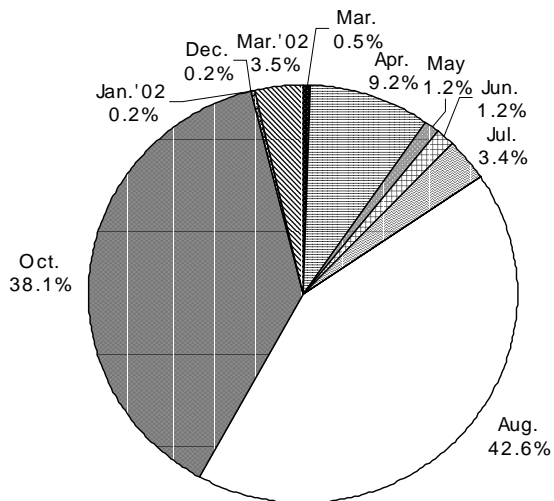
Fig. 5. Monthly variations in frequency of species occurrence (%) based on the number of individuals collected from the study area.
