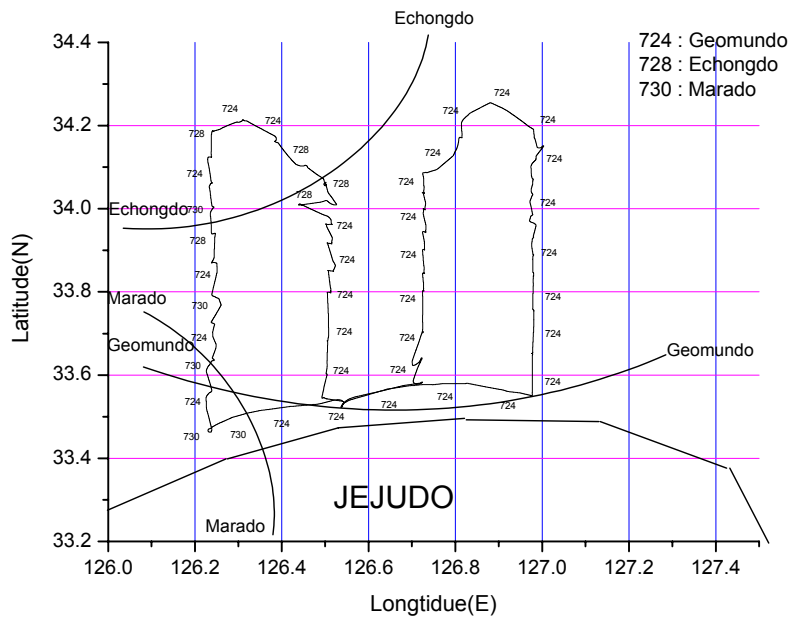
Fig. 6. ID's DGPS beacon stations obtained by DGPS receiver on the strait of Jeju from June 12 th to 15 th , 2002.
