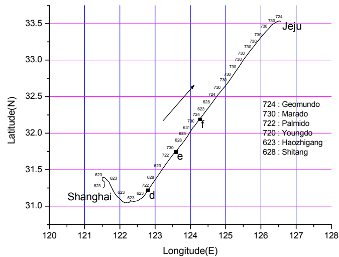
Fig. 8. ID's DGPS beacon stations obtained by DGPS receiver on Shanghai · Jeju route from October 13 th to 14 th , 2001.
