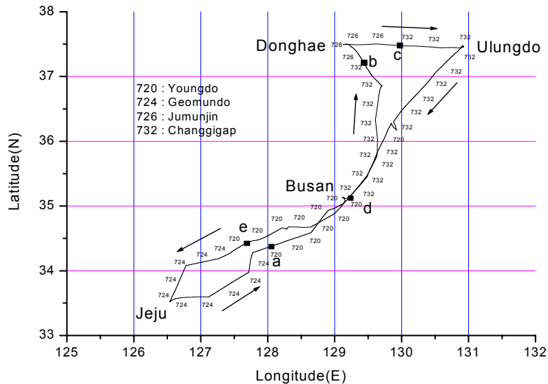
Fig. 18. ID's DGPS beacon stations obtained by DGPS receiver among Jeju, Busan, Donghae route from October 29 th to November 6 th , 2001.
