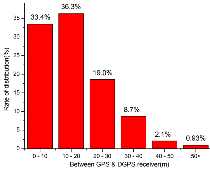
Fig. 21. The obtained of distance between GPS and DGPS receivers at the Jeju harbor.
