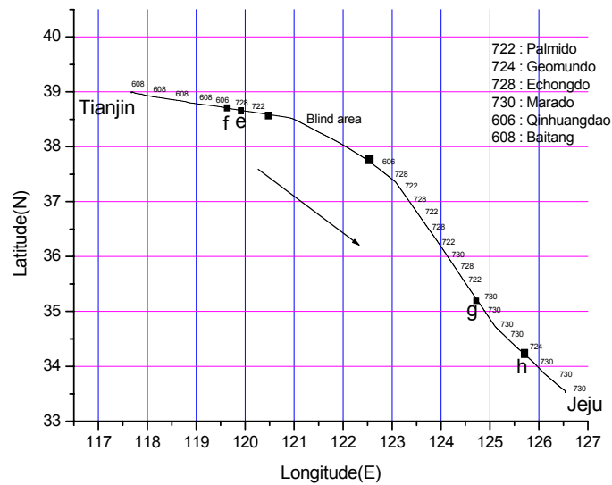
Fig. 10. ID's DGPS beacon stations obtained by DGPS receiver on Tianjin · Jeju route from June 29 th to July 1 st , 2002.
