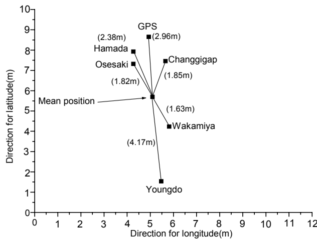
Fig. 36. The result V of position error obtained by DGPS and GPS receivers with Youngdo, Changgigap, Hamada, Osesaki and Wakamiya beacon stations for 5 minutes each at the mean position of Busan harbor.
