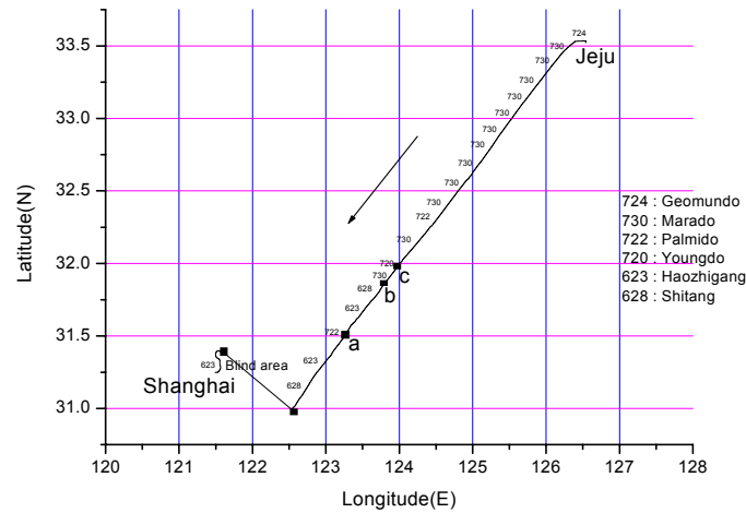
Fig. 7. ID's DGPS beacon stations obtained by DGPS receiver on Jeju · Shanghai route from October 7 th to 8 th , 2001.
