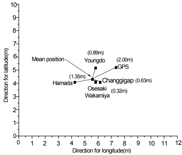
Fig. 35. The result IV of position error obtained by DGPS and GPS receivers with Youngdo, Changgigap, Hamada, Osesaki and Wakamiya beacon stations for 5 minutes each at the mean position of Busan harbor.
