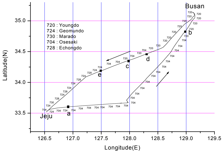
Fig. 17. ID's DGPS beacon stations obtained by DGPS receiver on Jeju · Busan route from September 25 th to 29 th , 2001.
