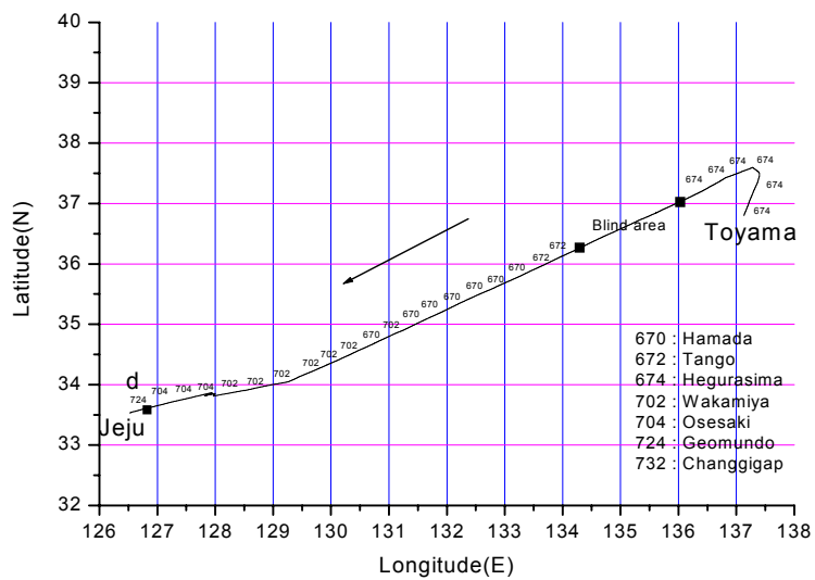
Fig. 14. ID's DGPS beacon stations obtained by DGPS receiver on Toyama · Jeju route from July 16 th to 18 th , 2002.
