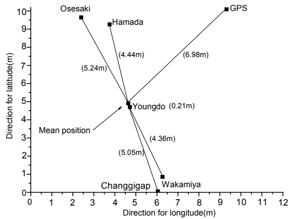
Fig. 33. The result II of position error obtained by DGPS and GPS receivers with Youngdo, Changgigap, Hamada, Osesaki and Wakamiya beacon stations for 5 minutes each at the mean position of Busan harbor.
