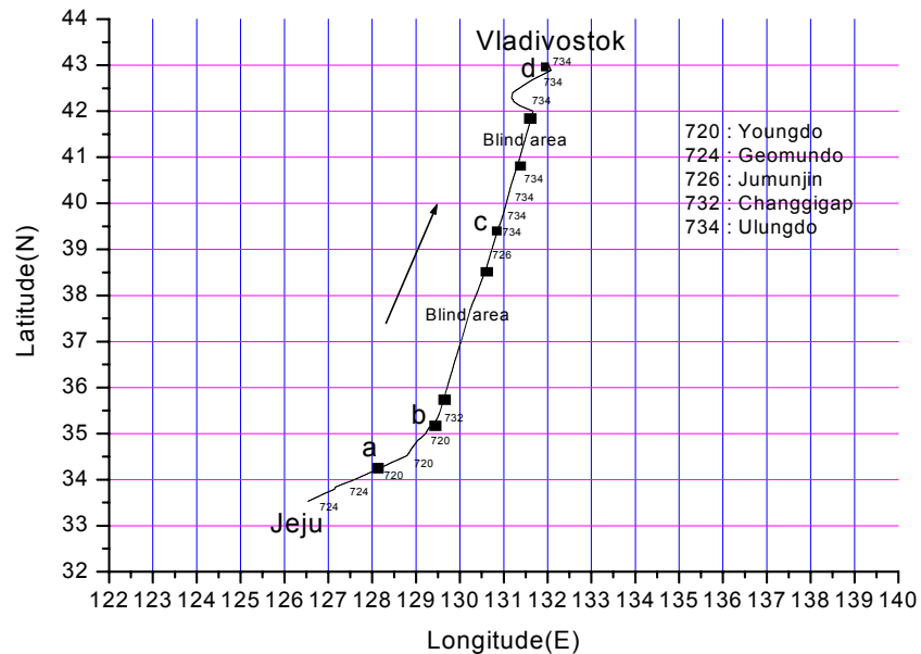
Fig. 15. ID's DGPS beacon stations obtained by DGPS receiver on Jeju · Vladivostok route from July 22 nd to 24 th , 2002.
