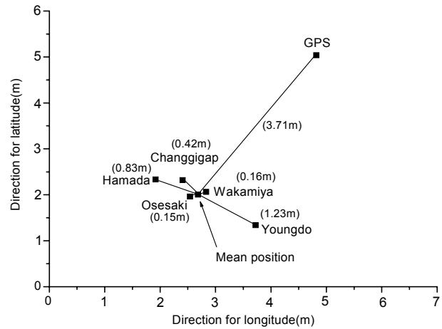
Fig. 29. Average of position error obtained by DGPS and GPS receivers with Youngdo, Changgigap, Hamada, Osesaki and Wakamiya beacon stations for 4 hours each at the mean position of Busan harbor from August 17 th to 18 th , 2002.
