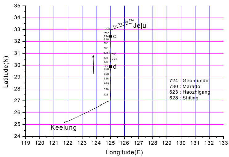
Fig. 12. ID's DGPS beacon stations obtained by DGPS receiver on Keelung · Jeju route from September 18 th to 21 st , 2001.
