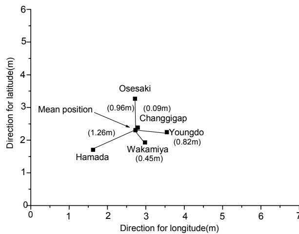
Fig. 31. Average of position error obtained by DGPS and GPS receivers with Youngdo, Changgigap, Hamada, Osesaki and Wakamiya beacon stations for 4 hours each at the mean position of Busan harbor from August 20 th to 21 st , 2002.
