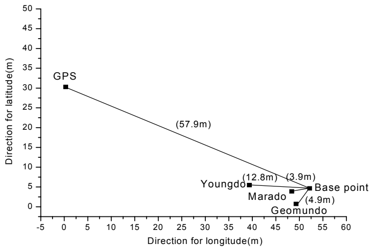
Fig. 22. Average of position error obtained by DGPS and GPS receivers with Geomundo and Marado beacon station at the base point of Sarabong.(Oct. 5 th , 2002)
