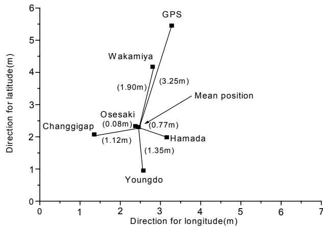
Fig. 27. Average of position error obtained by DGPS and GPS receivers with Youngdo, Changgigap, Hamada, Osesaki and Wakamiya beacon stations for 4 hours each at the mean position of Busan harbor from August 13 th to 14 th , 2002.
