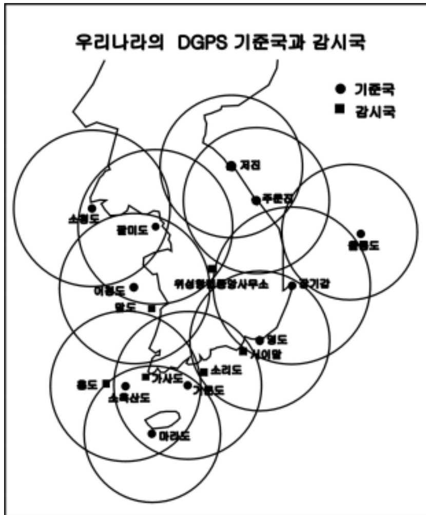
Fig. 2. DGPS beacon stations of Korea. (Reference stations and integrity stations)
