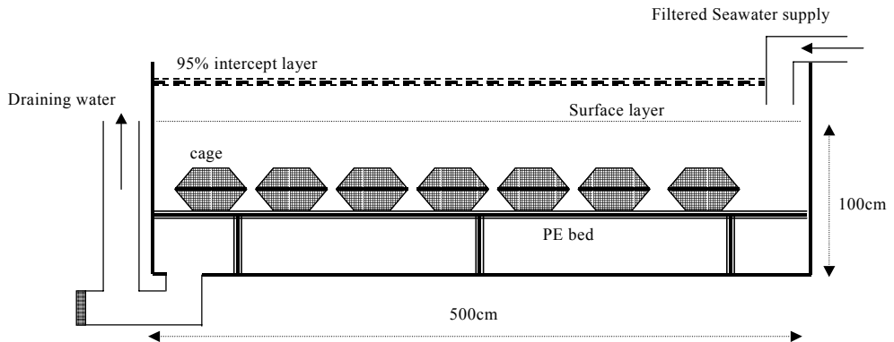
Fig. 2. Schematic representation of experimental containers in which small, medium and large abalone were housed during the experiment.
