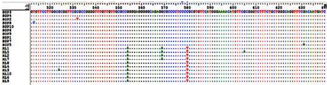
Fig. 11. Mutation patterns of nrITS gene sequences within Jeju Opuntia Genus populations (Bioedit program).
