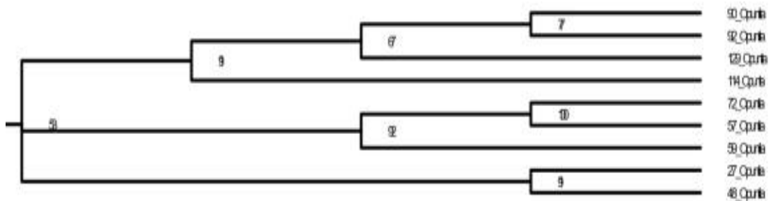
Fig. 21. Tree of nrITS and Plastid(rbcL and matK) Gene(with 92 Opuntia monacantha ) in Opuntia Genus registered in NCBI.
