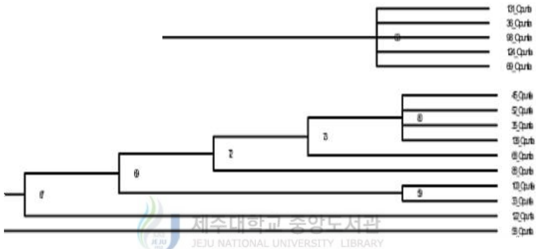
Fig. 22. Tree of Duplication clade's Gene.
