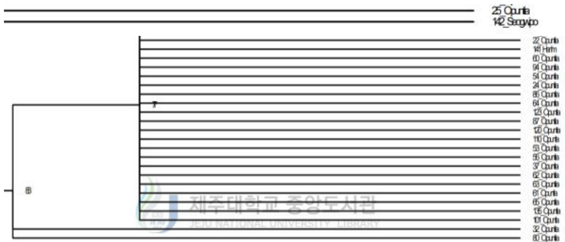
Fig. 15. Tree of nrITS Gene in Jeju Opuntia Genus and Opuntia Genus registered in NCBI (with 141 Hallim, 142 Seogwipo).
