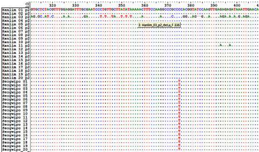
Fig. 14. Genetic variation pattern in rbcL gene between Jeju Opuntia Genus populations.
