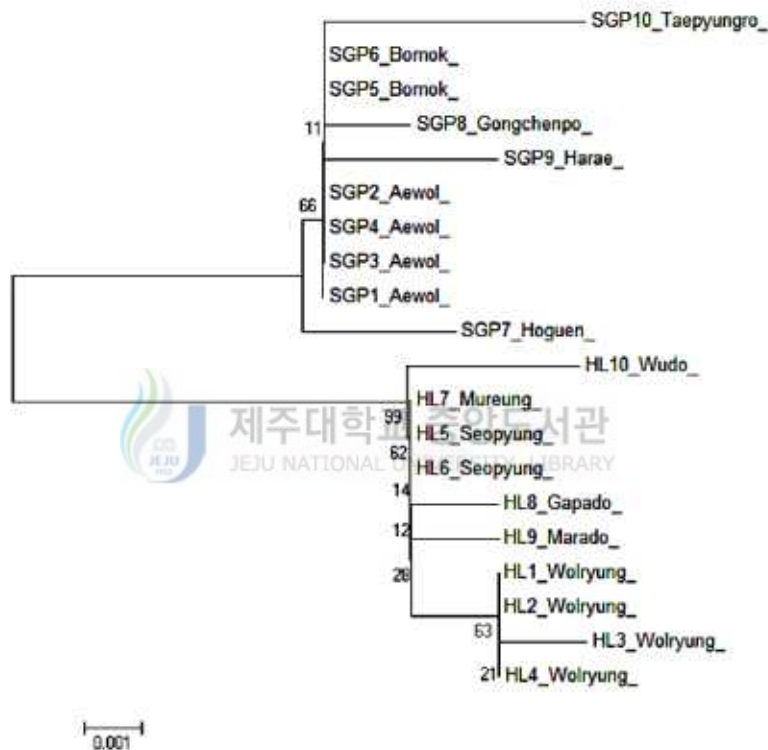
Fig. 12. Evolutionary relationships of taxa of Seogwipo and Hallim Opuntia (N) tree from the analysis of the nrITS).
