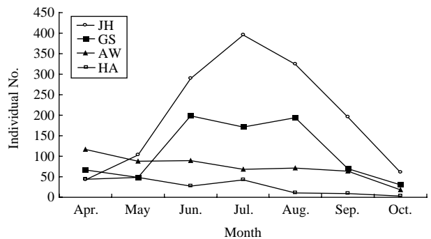
Fig. 2. Temporal change of the total individual numbers of four communities. Abbreviations of the legend represent the gotjawal terrains shown in Fig. 1.
