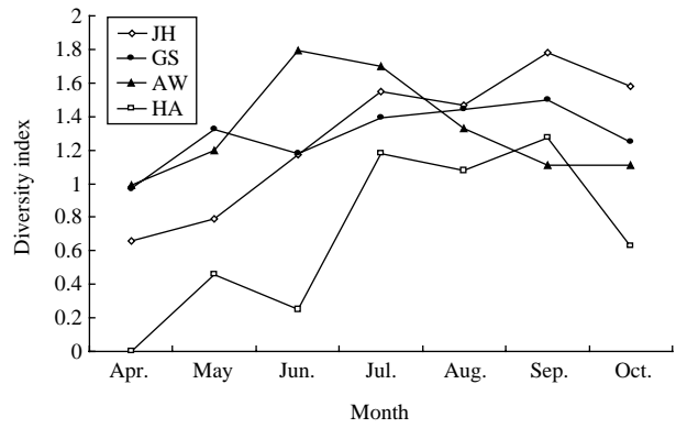
Fig. 5. Temporal change of the species diversity of four gotzawal communities.
